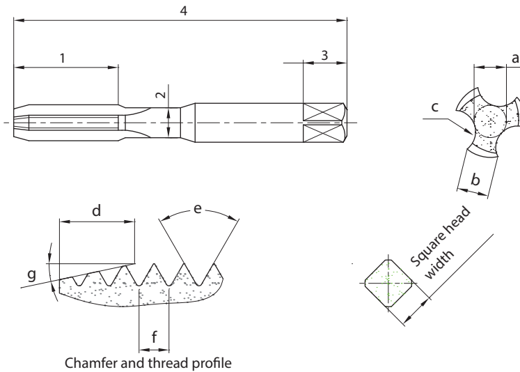
Chamfer and thread profile
