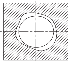
Roundness
